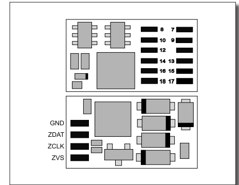
PluX12 interface
